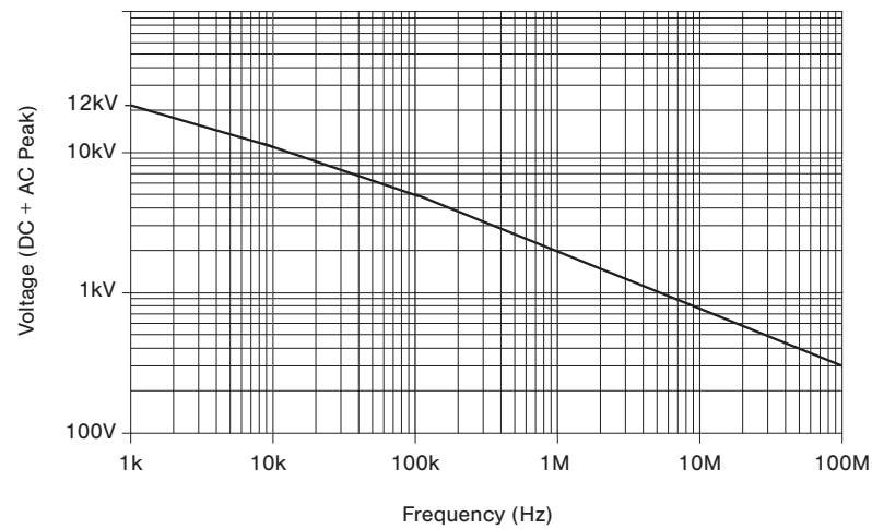
Figure 11 Voltage Derating Curve
